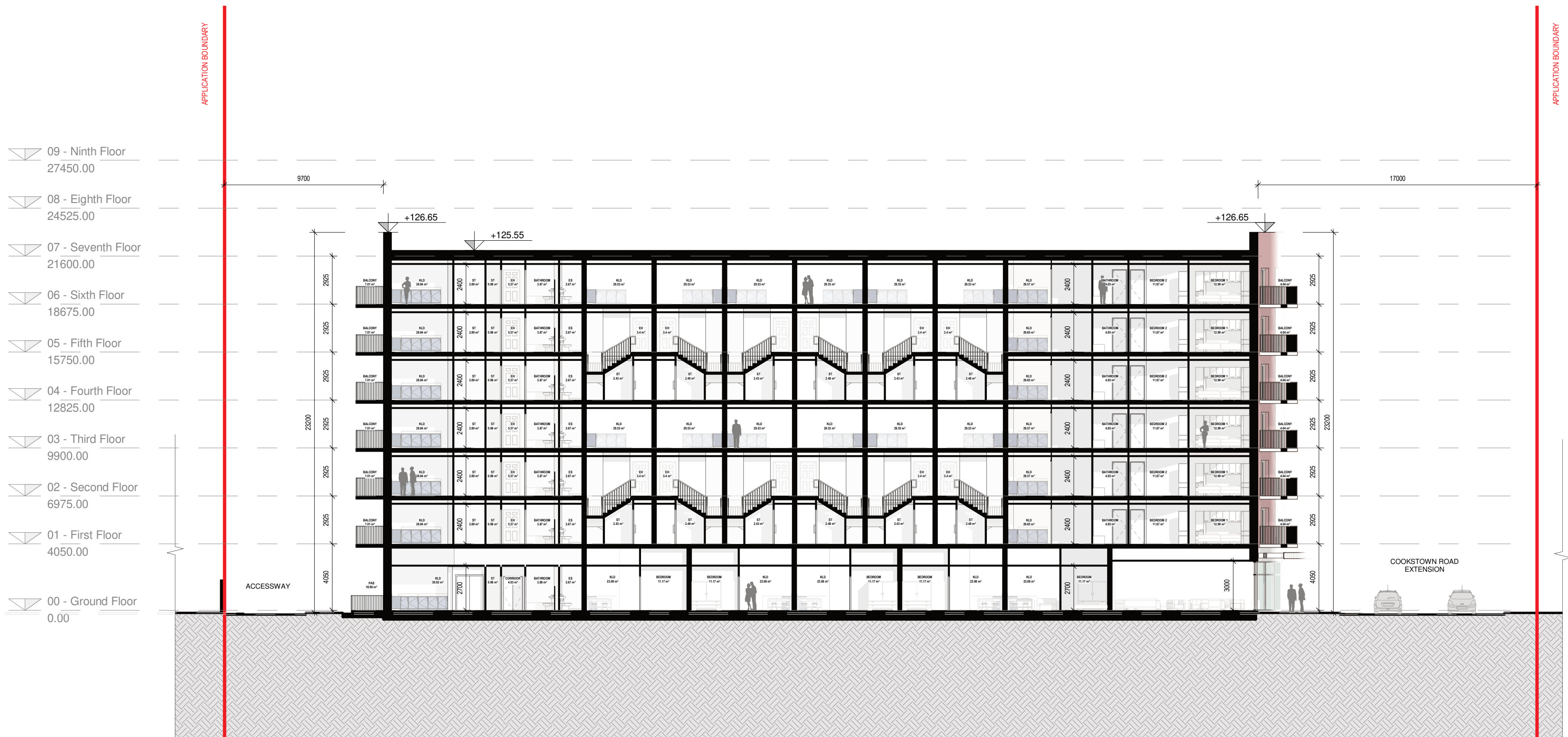
2 PROPOSED SECTION D - D 1 : 200
